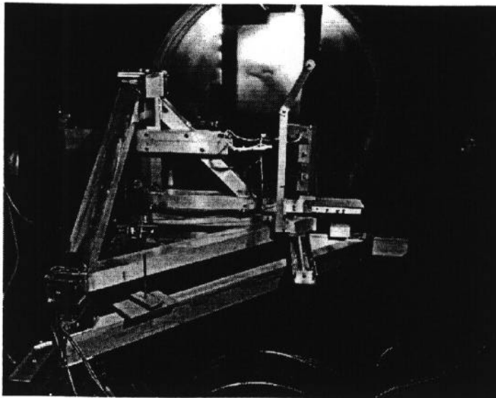
Figure 3: Photograph of Thrust Stand with Primex Breadboard PPT.
