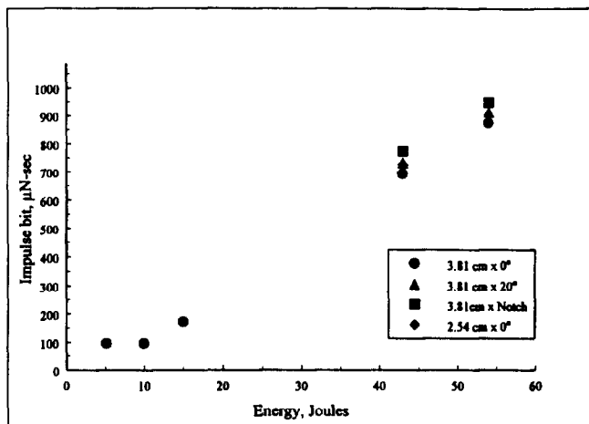
Figure 4: Impulse Bit versus Energy Level for Various Electrode Configurations.
