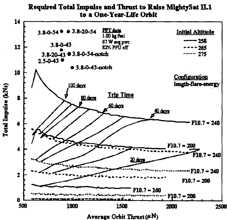
Figure 5: PPT Total Impulse Vs. Average Orbit Thrust Available reproduced from Reference 1.
