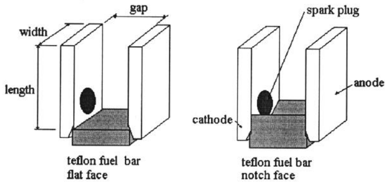
Figure 2: Schematic of Fuel Face and Electrode Configurations for a PPT.
