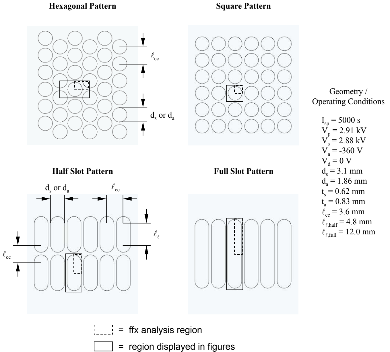
Figure 5. SUNSTAR grid aperture patterns.
