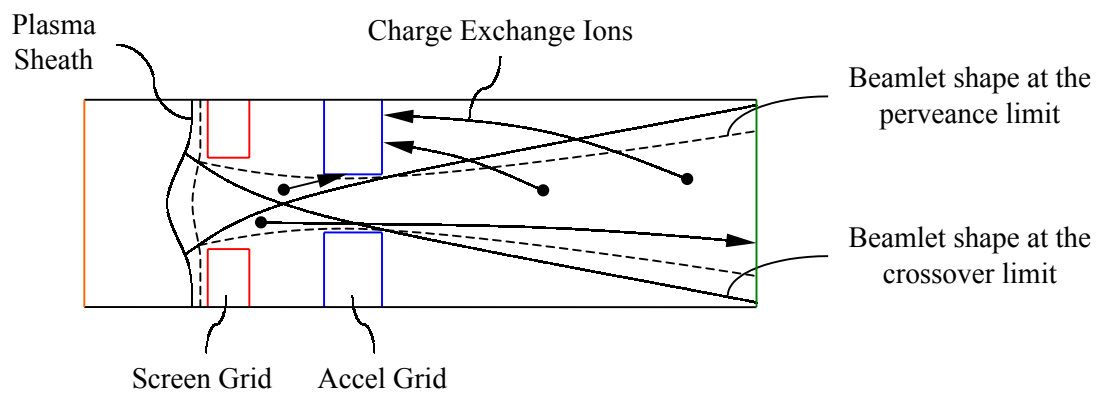
Figure 6. Perveance and crossover impingement limits.
