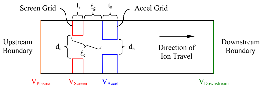
Figure 1. Typical two-grid thruster geometry.
