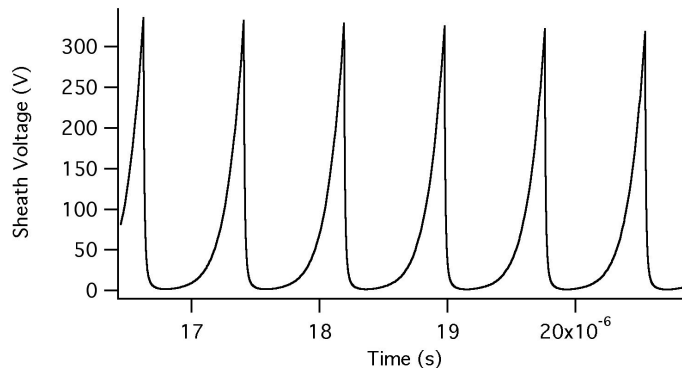
Figure 4. An example result of the sheath model. \beta = 6 , \Delta J = 5 A.
