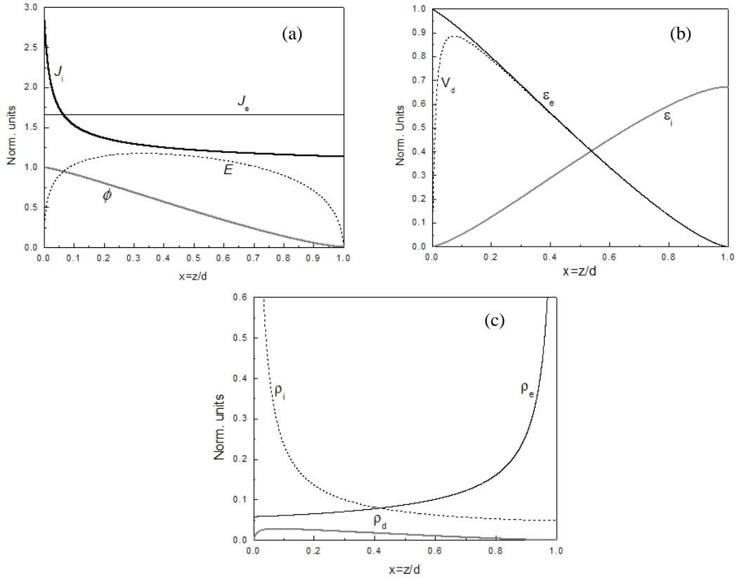
Fig. 4. Normalized axial distributions of: (a) the electron and ion current densities, the plasma potential, and the electric field, (b) the electron and ion energies, and the dust particle potential, (c) the electron, ion, and dust charge densities.
