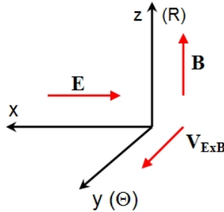
Fig. 5. The coordinate system for a Hall thruster in a slab geometry.
