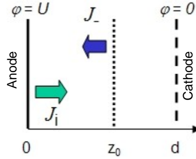
Fig. 1. Schematic of an ion thruster (ion diode) with negative ion injection from the intermediate electrode.
