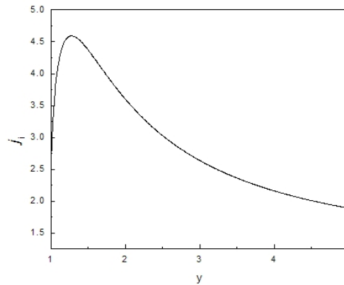
Fig. 2. Normalized ion current as a function of y defined in Eq. 9.
