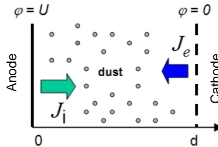
Fig. 3. Scheme of space charge neutralization with dust particles and an electron beam.
